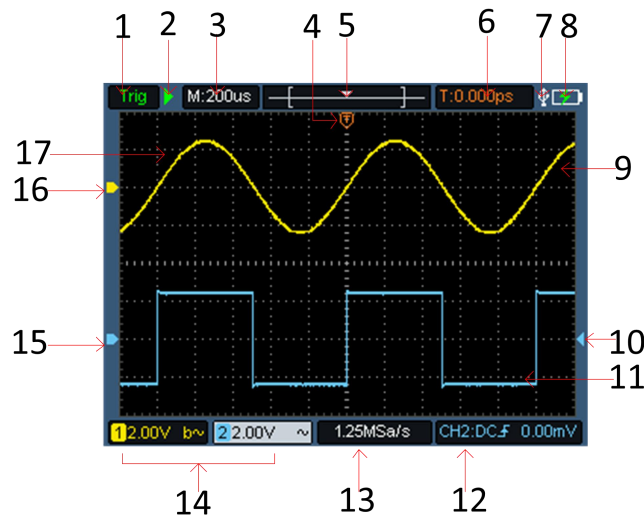
Figure 5: Oscilloscope Interface
