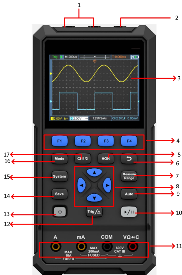
Figure 1: Front Panel of the Oscilloscope
