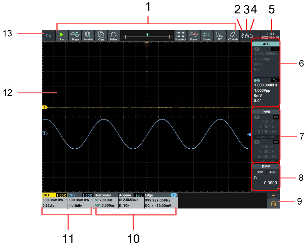
Figure 3-3: Illustrative Drawing of Display Interfaces
