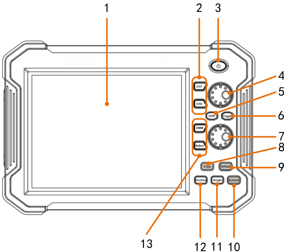
Figure 3-1 Front panel
